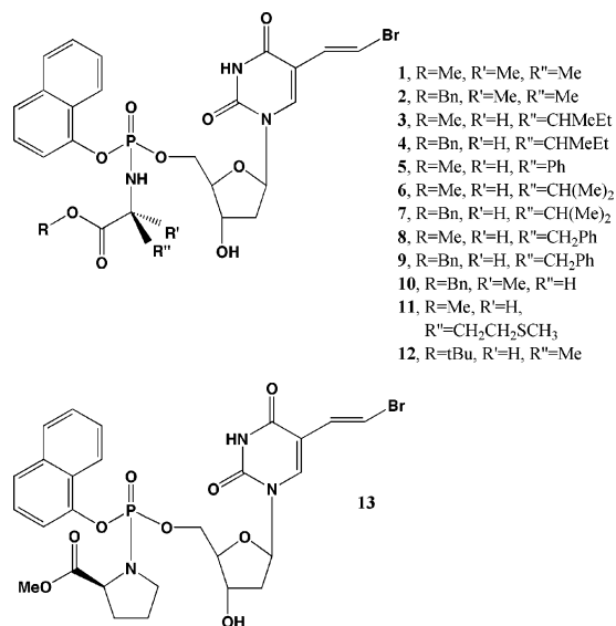
Scheme 1. Structures of 1–13
